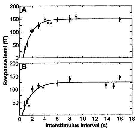
Fig. 1. Peak magnetic field strength near the scalp, \sim 100 ms after the onset of a tone-burst stimulus (the N100 component), increases with interstimulus interval, as shown for (A) the left hemisphere ( \tau = 1.3 s) and (B) the right hemisphere ( \tau = 1.5 s) of subject SW. The field sensor was placed over each hemisphere at a location where it monitors activity in the primary auditory cortex.
